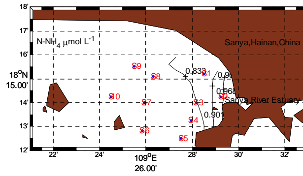
(a) Spatial distribution of the annual concentration of \text{N-NH}_4 .
