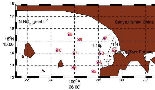
(b) Spatial distribution of the annual concentration of \text{N-NO}_3 .
