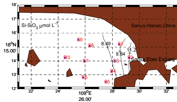
(c) Spatial distribution of the annual concentration of \text{Si-SiO}_3 .
